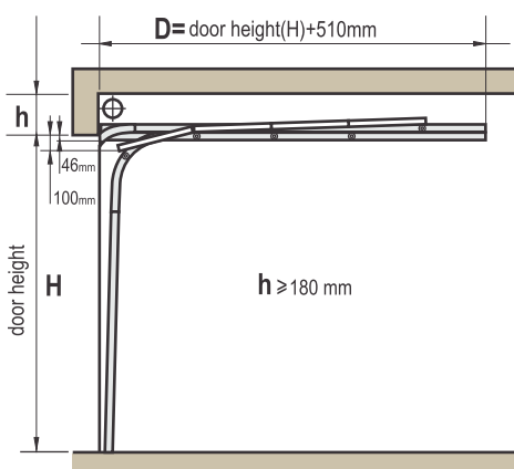
LHR FM - low headroom lift double tracks, front mounted springs
