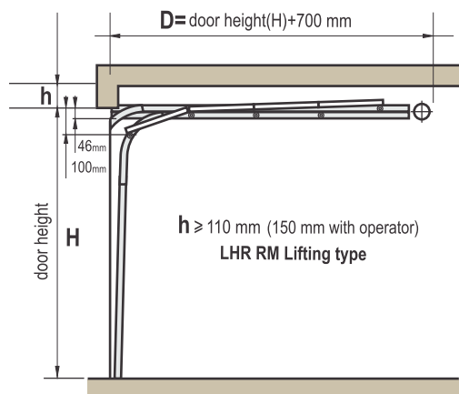
LHR RM - low headroom lift double tracks, rear mounted springs
